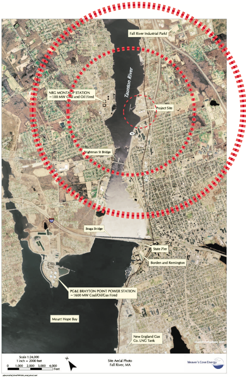
Figure 2: The thermal radiation danger zones for spills listed in Table 2. Red circles are distances to radiation intensities of 1.6 \text{ kW/m}^2 for a spill with fire. Largest circle is for failure of secondary tank containment; next smaller for tanker hold contents; smallest for loss of primary containment.
