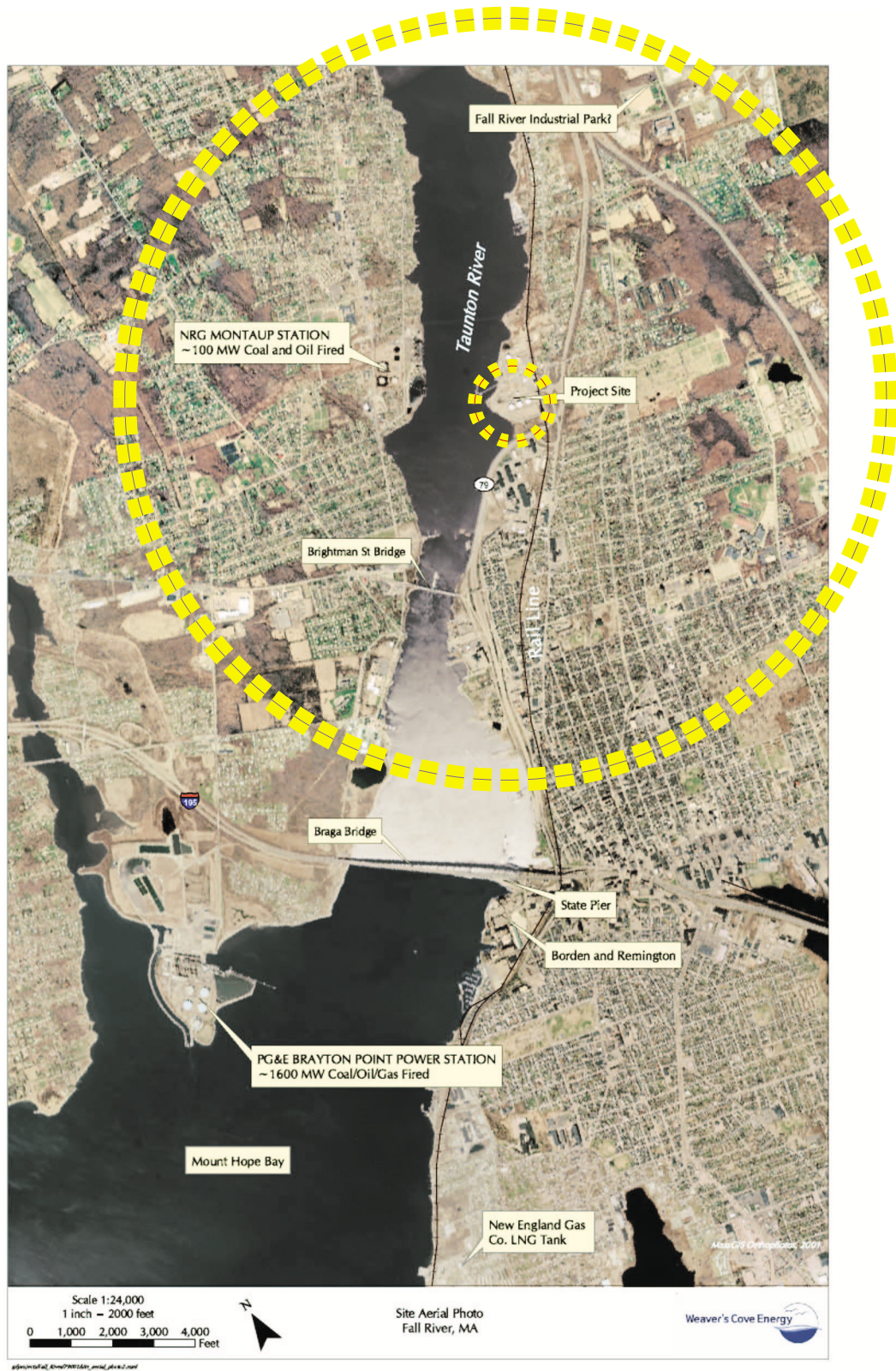
Figure 4: The flammable vapor danger zones for on-site spills without fire. The large circle is for a loss of primary containment; the small, for a transfer piping spill.
